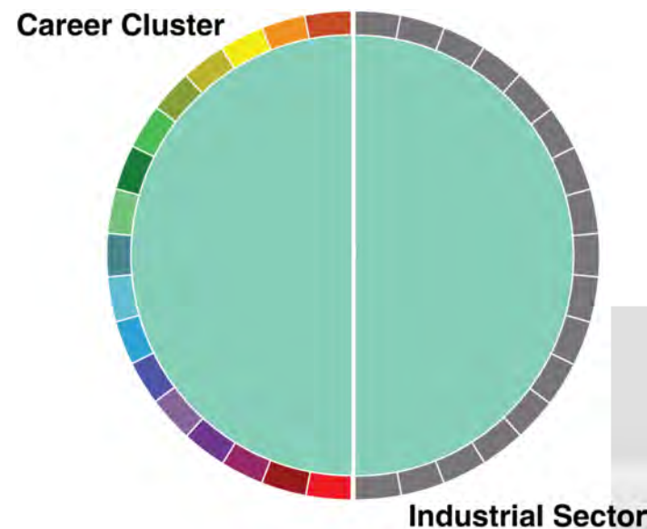
Figure 1. Circos illustration.
